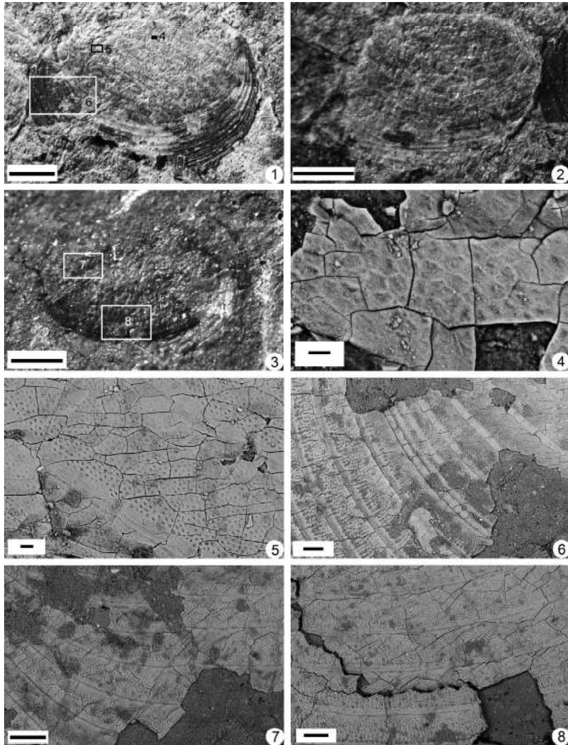
Fig. 4. 1–8. Linglongtaesthesia daxishanensis gen. and sp. nov. 1, a right valve, NIGPCAS 163668 (L2–1) (light microscopy). 2, a broken right valve, NIGPCAS 163669 (L2–2) (light microscope). 3, displaced carapaces, NIGPCAS 163670 (L2–3) (light microscope). 4, small-sized polygonal reticulation on growth bands near the umbo of the specimen in figure 4.1 (SEM). 5, evenly distributed puncta in the middle part of the carapace of the specimen in figure 4.1, i.e. , puncta in the upper and radial lirae with intercalated radially aligned puncta in the lower part of each growth band (SEM). 6, two kinds of ornamentation pattern on growth bands in the postero-ventral part of the carapace of the specimen in figure 4.1, i.e. , puncta in the upper and radial lirae with intercalated radially aligned puncta in the lower part of each growth band (SEM). 7, small-sized polygonal reticulation on growth bands in the antero-dorsal part of the carapace of the specimen in figure 4.3 (SEM). 8, two kinds of ornamentation pattern on growth bands in the ventral part of the carapace of the specimen in figure 4.3, i.e. , puncta in the upper part and radial lirae with intercalated radially aligned puncta in the lower part of each growth band (SEM). Scale bars: (1–3) = 1 mm; (4) = 10 \mu m; (5) = 20 \mu m; (6–8) = 100 \mu m.
