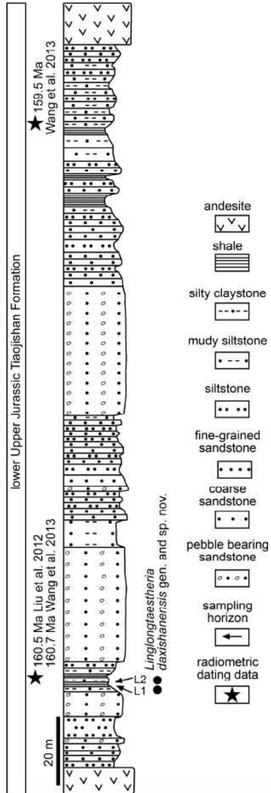
Fig. 2. Stratigraphic column of the Tiaojishan Formation exposed near Daxishan village, Linglongta, Jianchang County, showing the fossil clam shrimp sampling horizons (after Duan et al. 2009).
