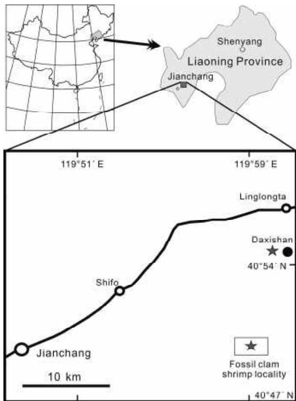
Fig. 1. Sampling locality at Daxishan village, Linglongta, Jianchang County, western Liaoning Province, China.
