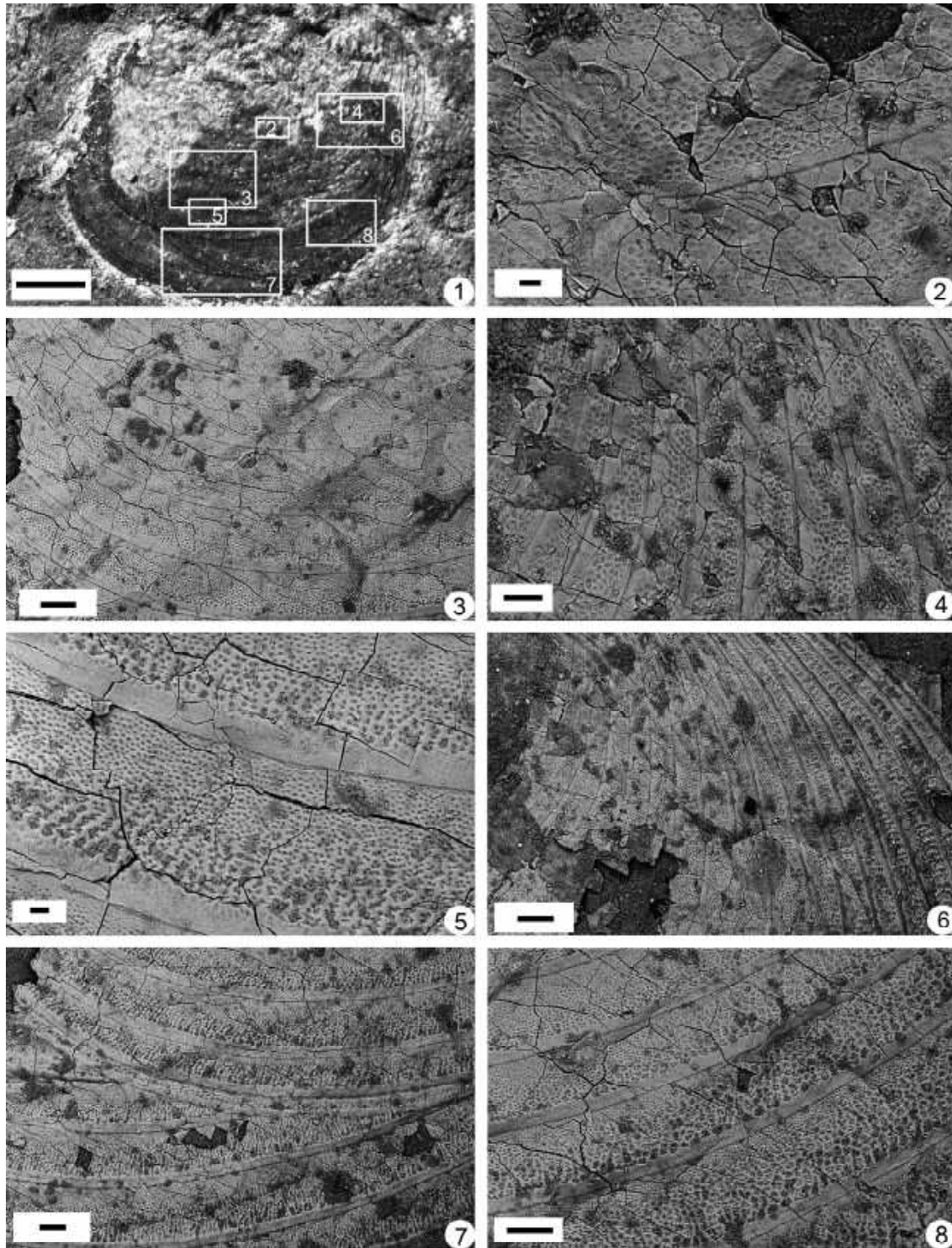
Fig. 3. 1–8. Linglongtaesthesia daxishanensis gen. and sp. nov. 1, displaced carapaces, holotype, NIGPCAS 163667 (L1–1) (light microscopy). 2, small-sized polygonal reticulation on growth bands near the umbo (SEM). 3, evenly distributed small puncta on growth bands in the middle part of the carapace (SEM). 4, small-sized polygonal reticulation on growth bands in the antero-dorsal part of the carapace (SEM). 5, 7, two kinds of ornamentation pattern on growth bands in the postero-ventral part of the carapace, i.e. , punctate ornamentation in the upper, radial lirae with two rows of intercalated radially aligned puncta in the lower part of each growth band (SEM). 6, small-sized, polygonal reticulation transitions to radial lirae with intercalated radially aligned puncta on growth bands in the antero-dorsal part of the carapace (SEM). 8, two kinds of ornamentation pattern on single growth bands in the antero-ventral part of the carapace, i.e. , puncta in the upper, punctate small-sized reticulation in the lower part of each growth band (SEM). Scale bars: (1) = 1 mm; (2, 5) = 20 \mu m; (4) = 50 \mu m; (3, 6–8) = 100 \mu m.
