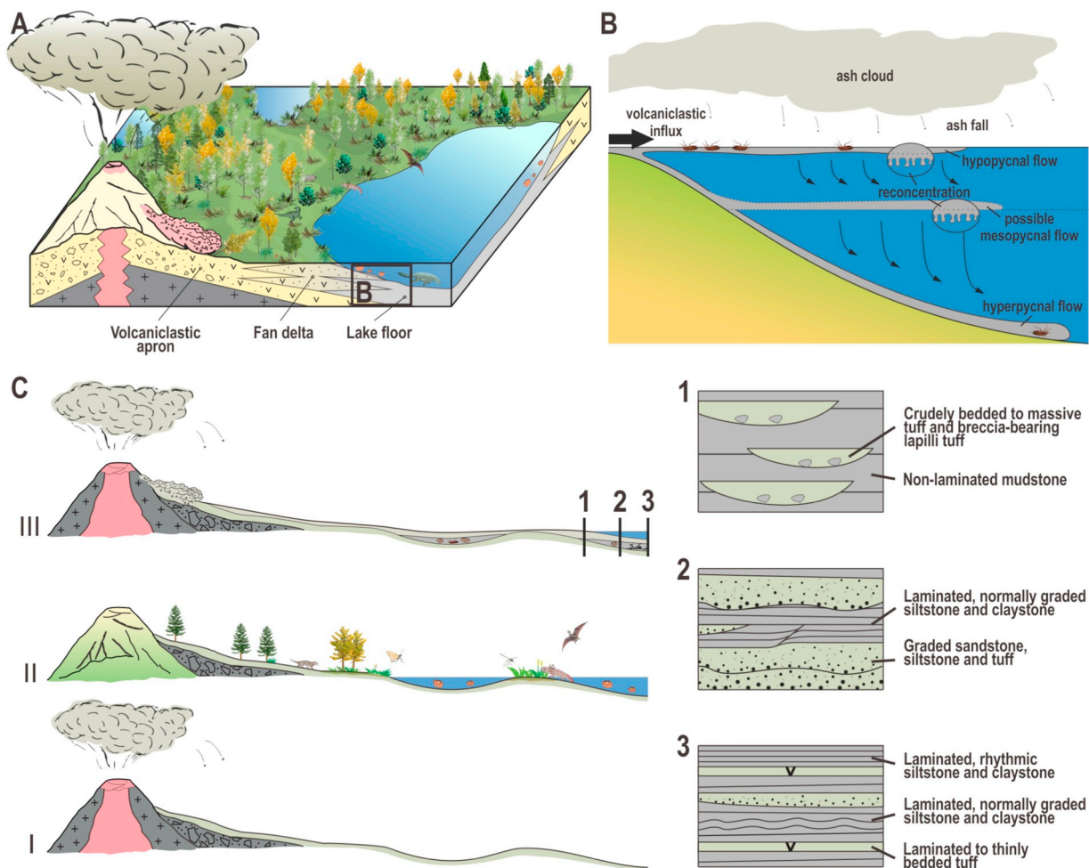
Fig. 7. A–B. Depositional model of the Daohugou Beds in the studied area (A), and biostratigraphic model of the land animal remains (B). C. Illustrative sketch (not to scale) of the evolution of the Daohugou lake(s): I–II, waterbodies gradually accumulated on the volcaniclastic apron, where the Daohugou ecosystem was established and developed; II–III, during syneruption periods, volcanoclastic influxes repeatedly devastated the ecosystem and buried the remains, and may even have destroyed the lake completely; keys as in Figs. 2 and 3. Some of the animal figures were revised from reconstructions by Rongshan Li, Nobu Tamura and April M. Isch.
