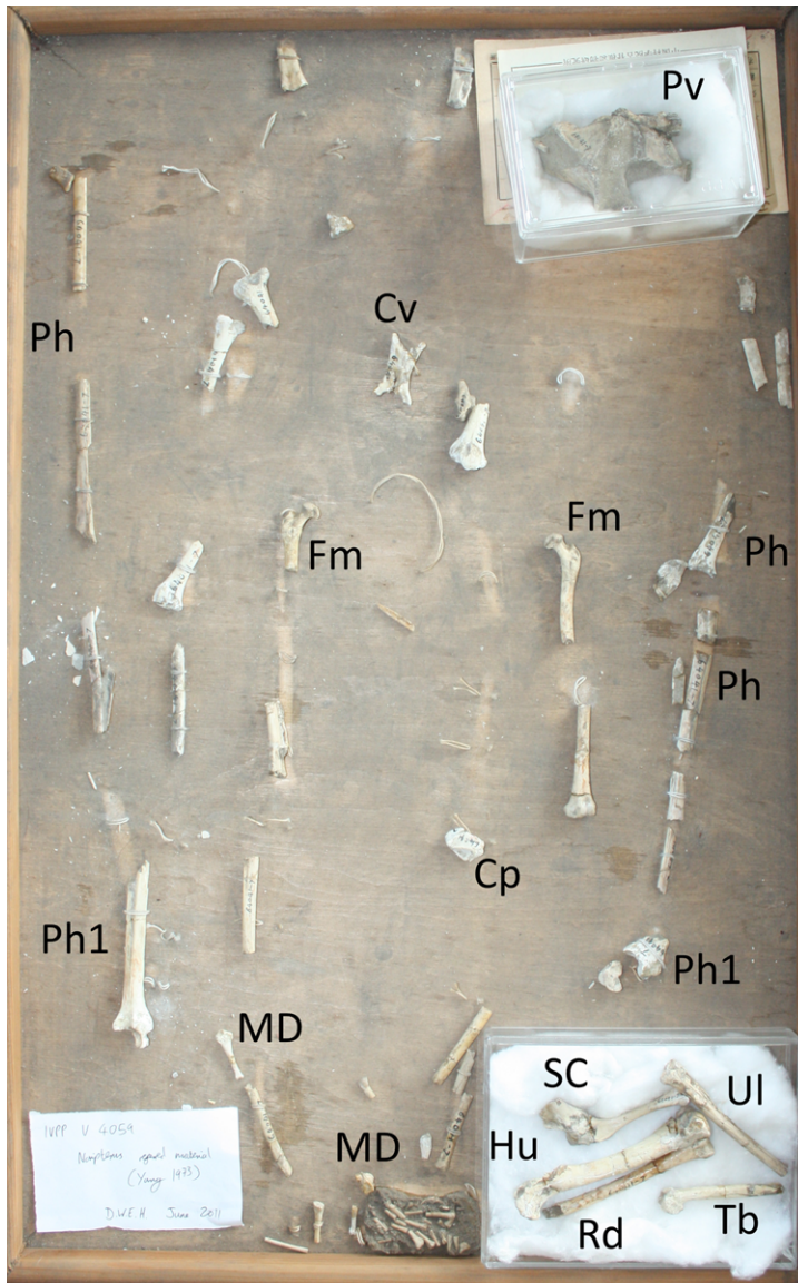
Fig. 3. The material belonging to specimen IVPP V 4059 of Noripterus (field number 64041-7) as found in the collections with material mounted on a wooden board – note that in many cases long bones are broken and parts are missing but their original position and size can often be identified based on the cleaner parts of the board. Abbreviations as in Figure 2 with the following additions: Cv, cervical vertebra; MD, manual and/or pedal elements; Pv, pelvis; SC, scapulocoracoid. Not all elements are identified or labelled here.
